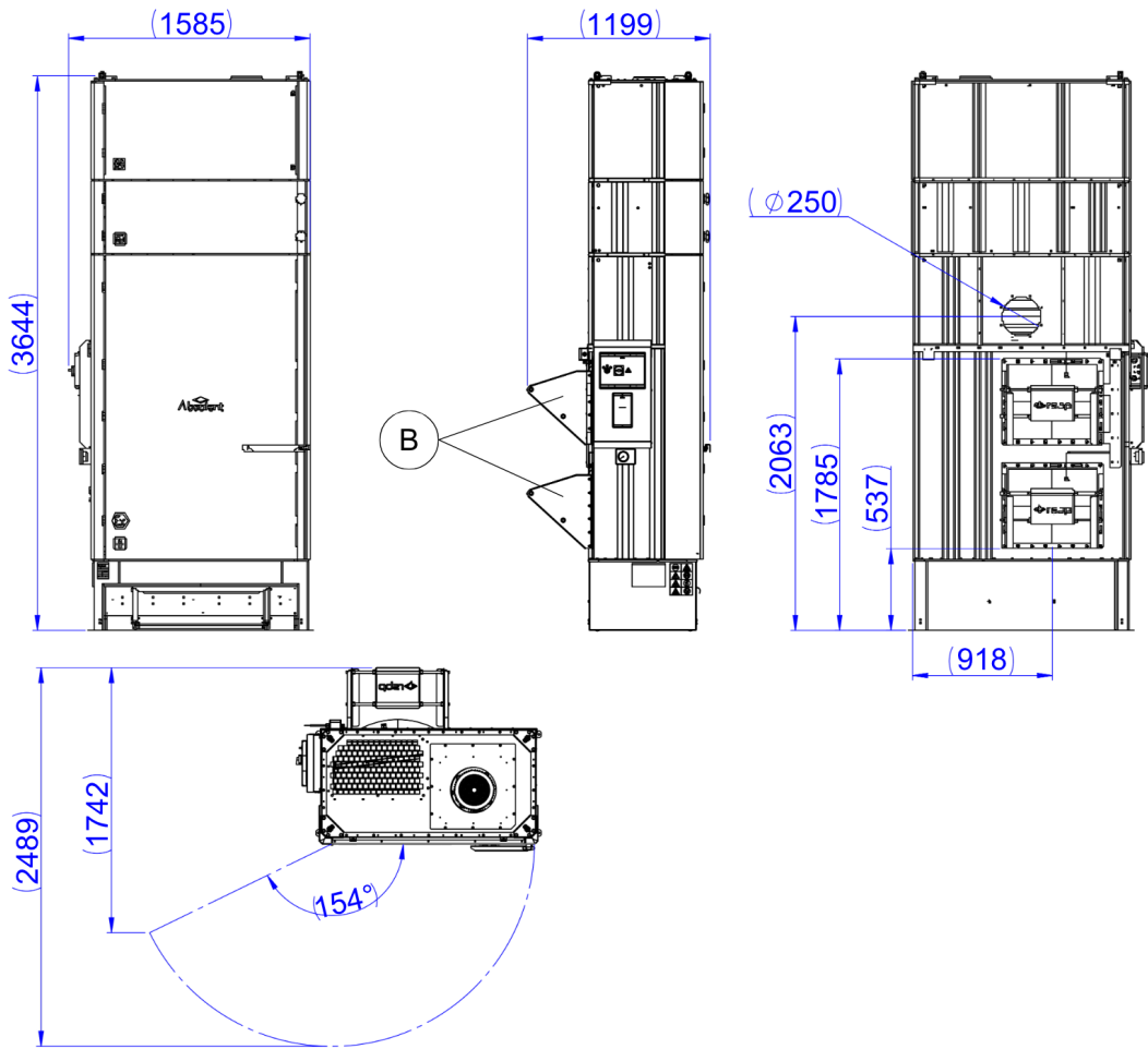
AD051EX with integrated fan, two explosion diverters (B) and HEPA module.
