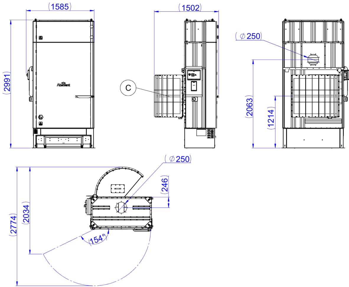
AD051EX with external fan, HEPA module and and a flameless vent (C).
