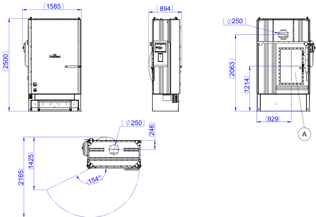
AD051EX with external fan and a single explosion panel (A).
