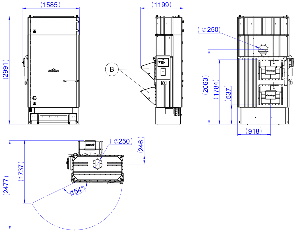
AD051EX with external fan, two explosion diverters (B) and HEPA module.
