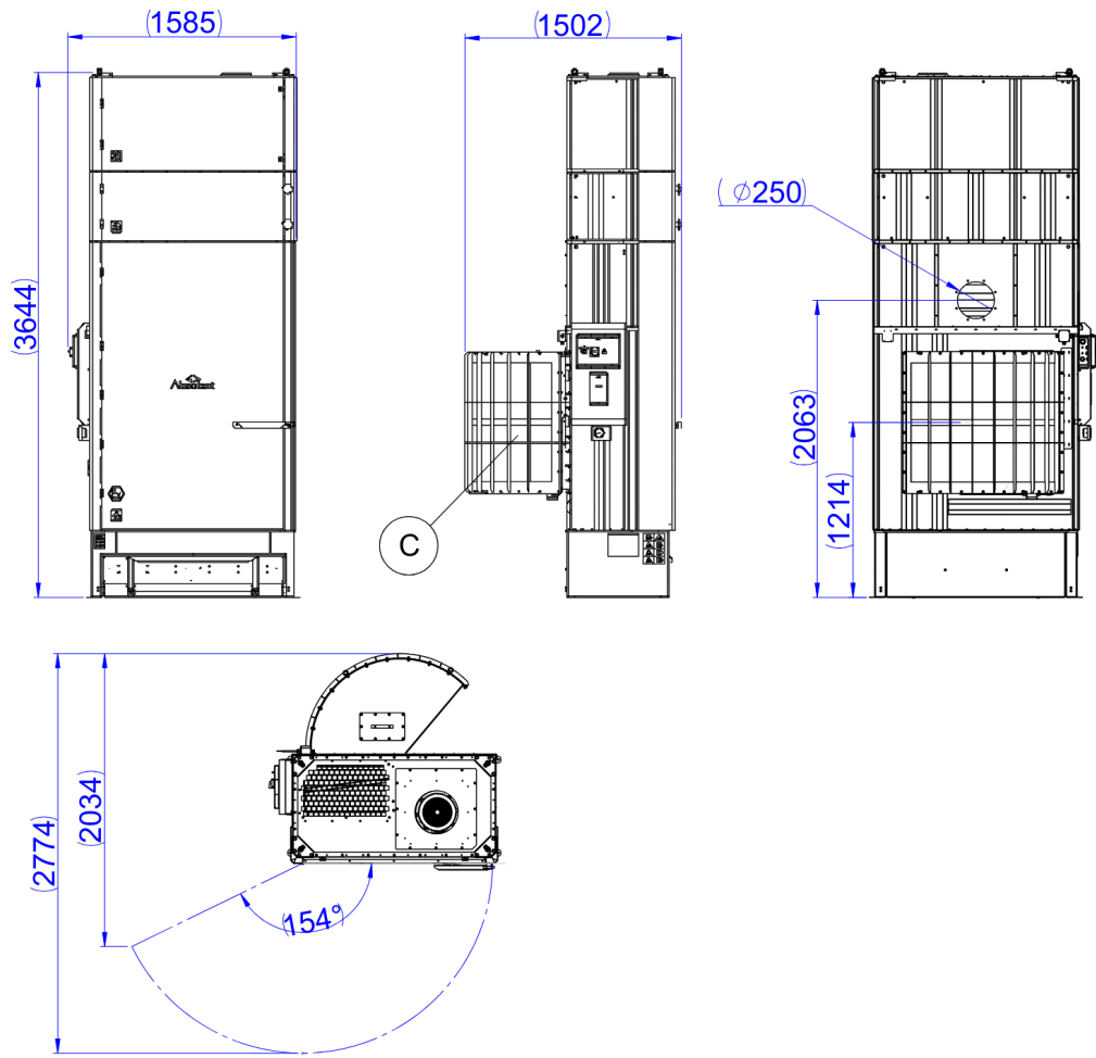
AD051EX with integrated fan, HEPA module and a flameless vent (C).
