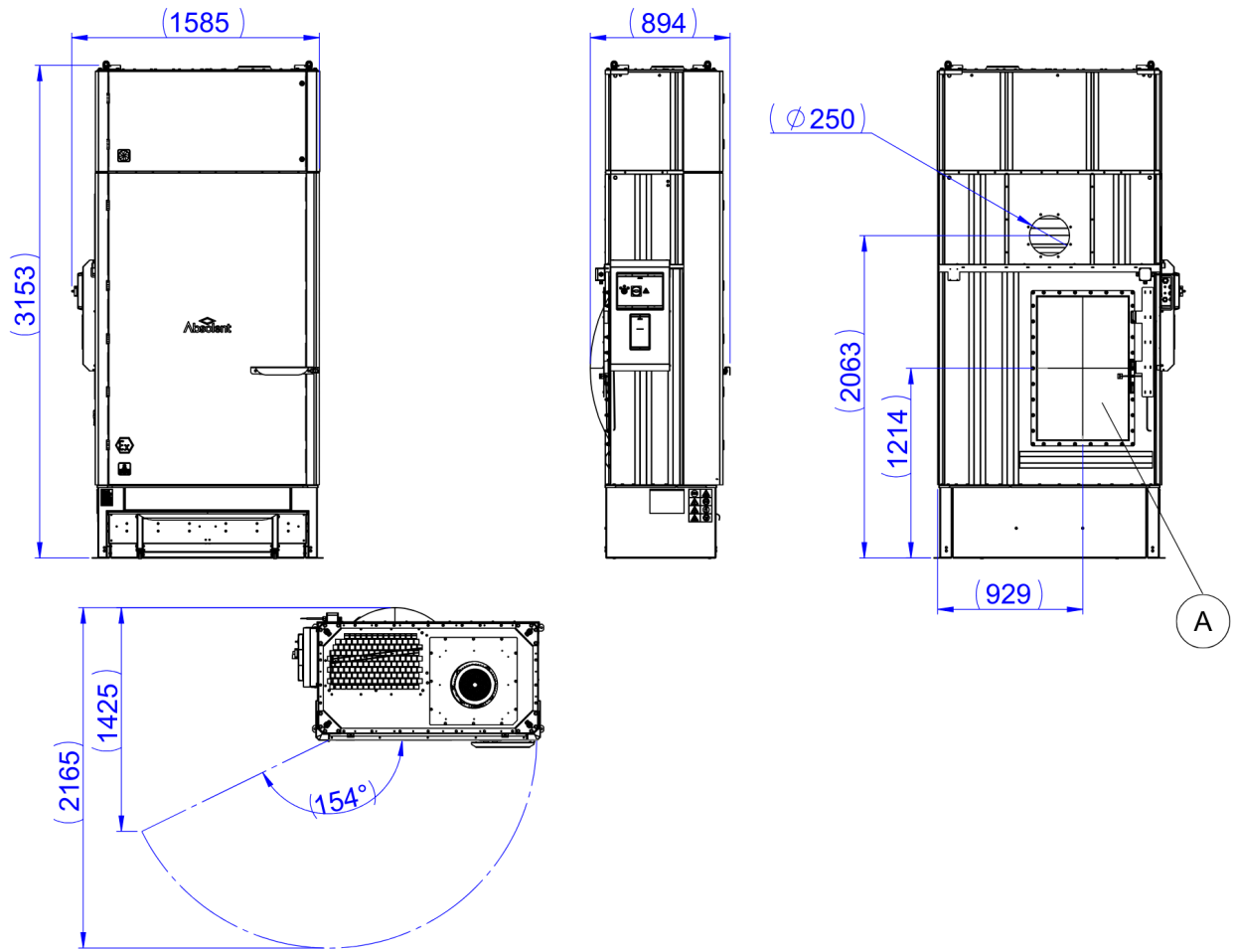
AD051EX with integrated fan and a single explosion panel (A).
